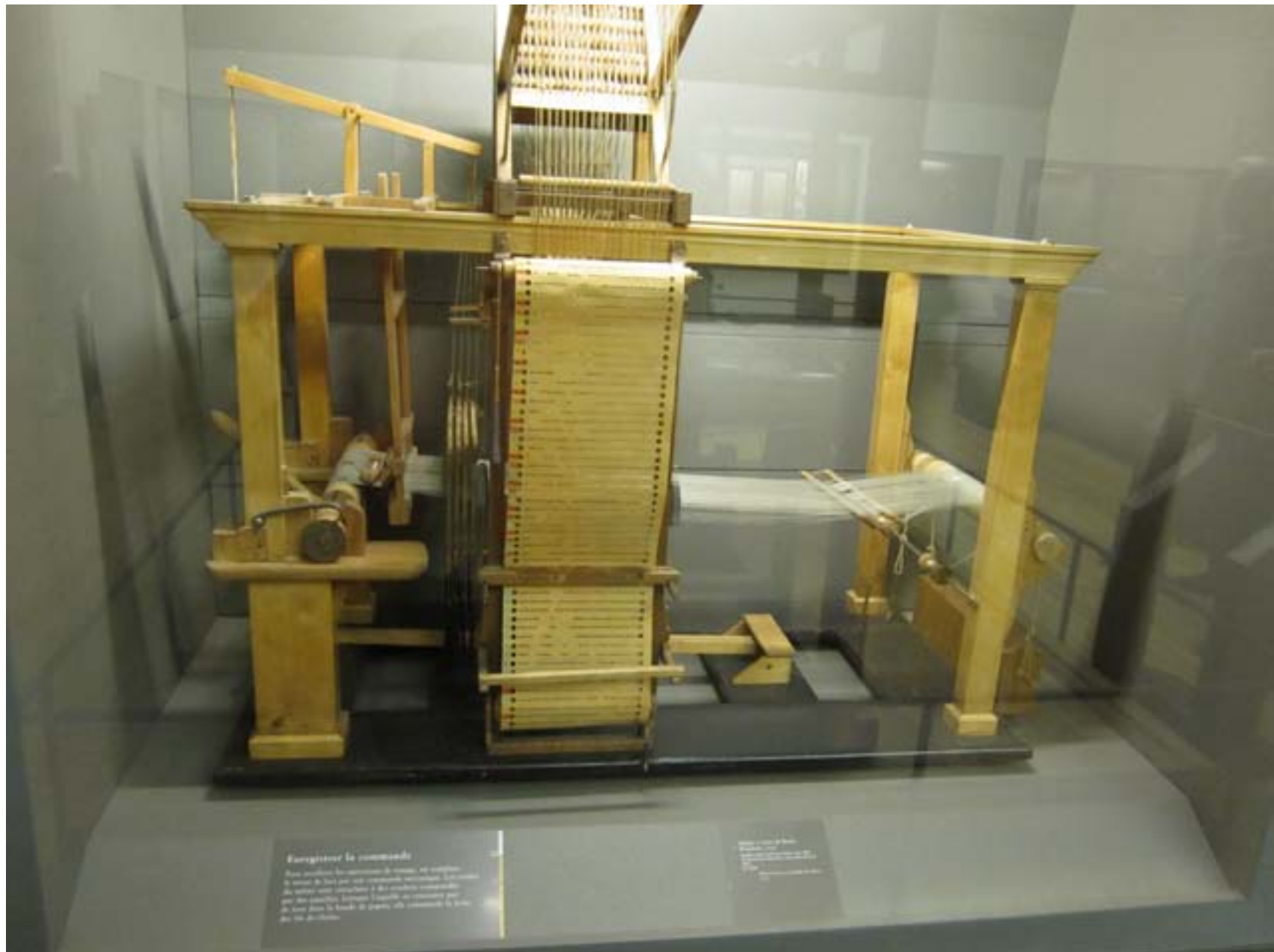
Ruban perforé - Basile Bouchon - 1725
